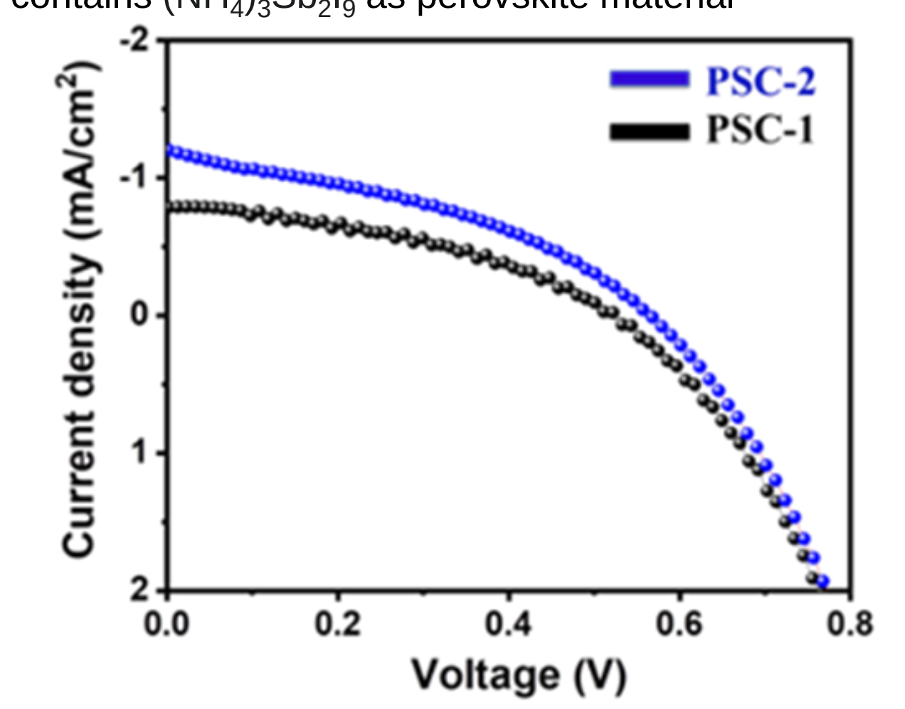
Fig. J-V curves of PSC-1 and PSC-2
