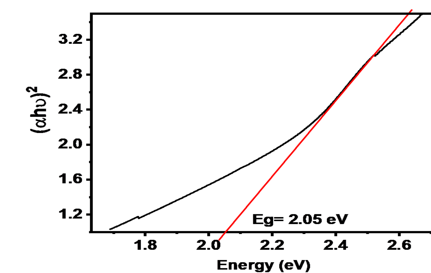
Fig. Tauc plot of (\text{NH}_4)_3\text{Sb}_2\text{I}_9
