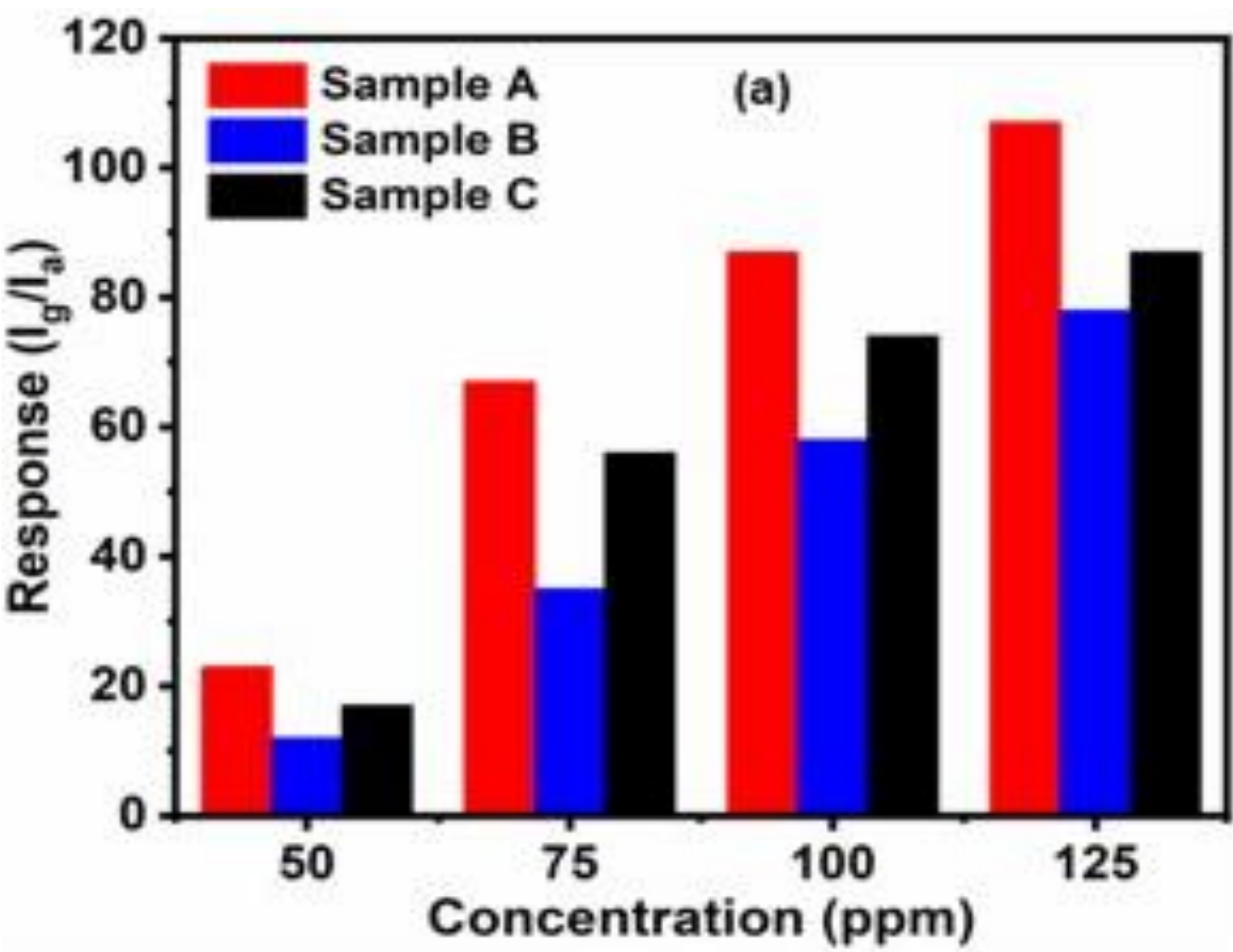
RESPONSES OF THREE SAMPLES AGAINST DIFFERENT CONCENTRATIONS OF ETHANOL
