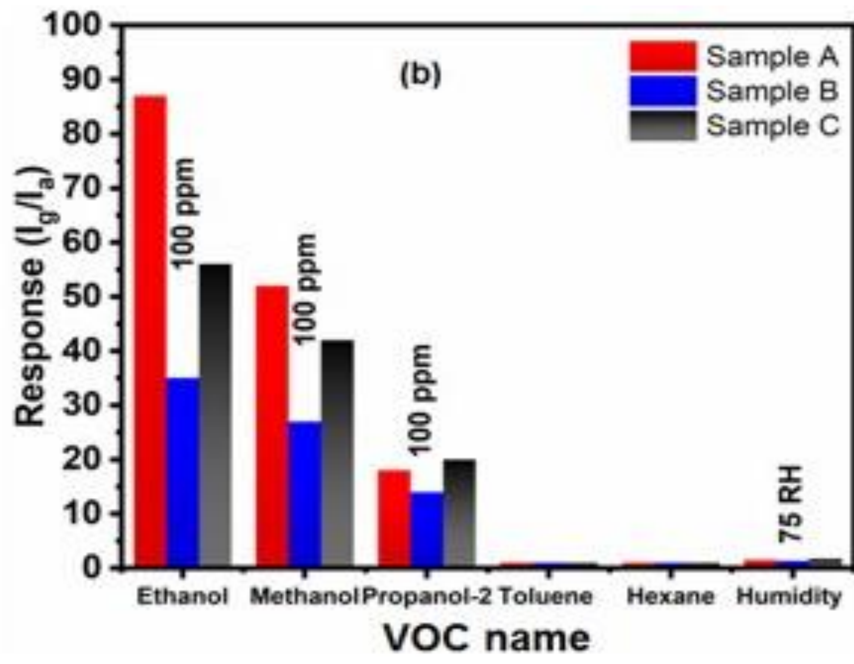
AGAINST 100 ppm OF DIFFERENT VOCs
